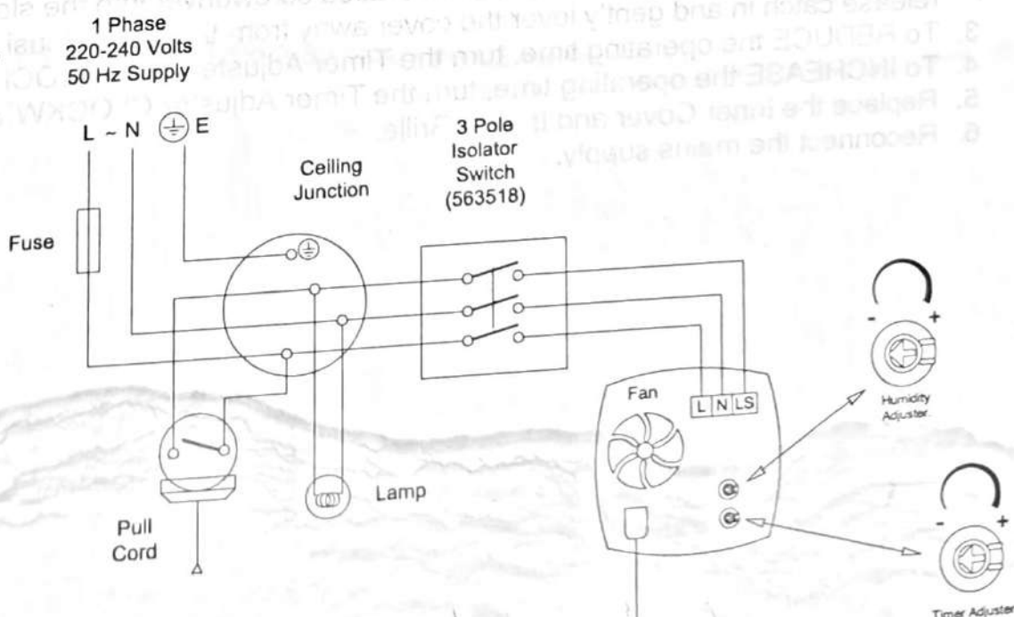
Fig. 6. VA140/150HT Humidity Timer Model. (140420A, 151420A WL, 150420A WW)
